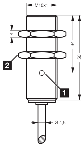
1) LED 2) Width over flats 24 mm BK: black BN: brown BU: blue
