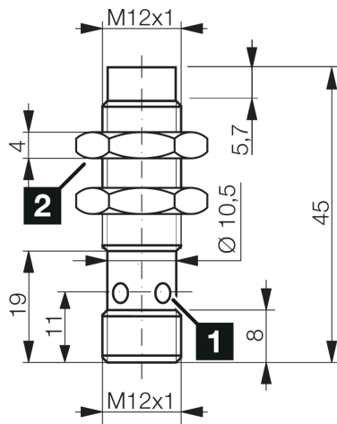
1) LED 4 x 90° (yellow) 2) Width over flats 17 mm BN: brown BU: blue WH: white
