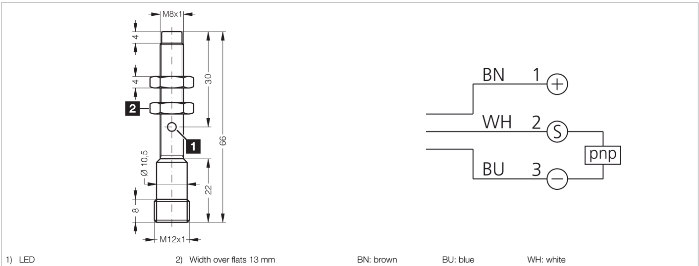
1) LED 2) Width over flats 13 mm BN: brown BU: blue WH: white
