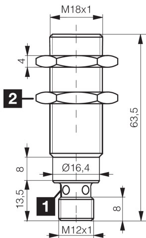
1) LED 4 x 90° (yellow) 2) Width over flats 24 mm BN: brown BU: blue WH: white
