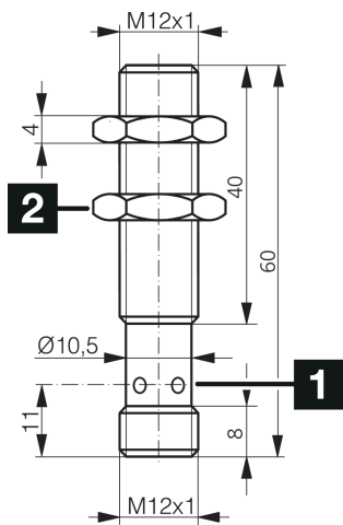
1) LED 4 x 90° (yellow) 2) Width over flats 17 mm BN: brown BU: blue WH: white
