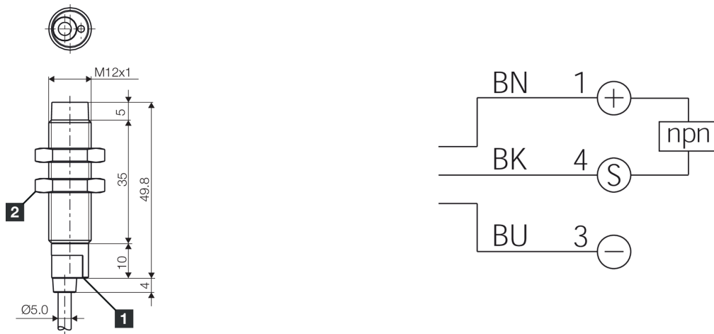
1) LED 2) Width over flats 17 mm BK: black BN: brown BU: blue
