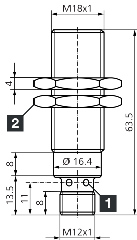
1) LED 4 x 90° (yellow) 2) Width over flats 24 mm BK: black BN: brown BU: blue
