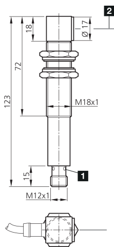
1) LED 4 x 90° (yellow) 2) Sound outlet ultrasonic transducer BK: black BN: brown BU: blue WH: white
