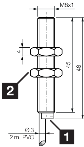
1) LED 2) Width over flats 13 mm BK: black BN: brown BU: blue
