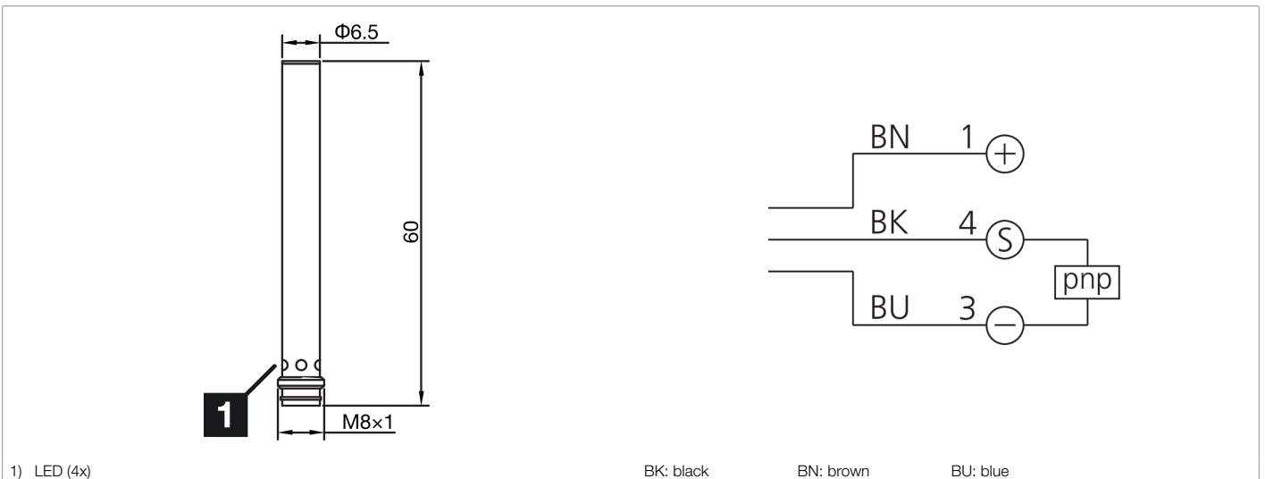
1) LED (4x)
