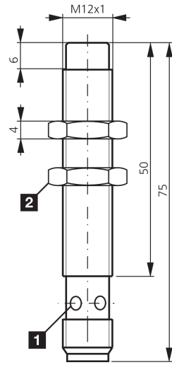
1) LED 4 x 90° (gelb) / LED 4 x 90° (yellow) / LED 4 x 90° (jaune) 2) Schlüsselweite 17 mm / Width over flats 17 mm / Ouverture de clé 17 mm mm
