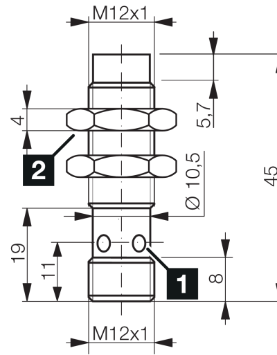
1) LED 4 x 90° (gelb) / LED 4 x 90° (yellow) / LED 4 x 90° (jaune) de clé 17 mm 2) Schlüsselweite 17 mm / Width over flats 17 mm / Ouverture de clé 17 mm
