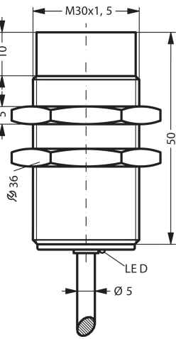
1) LED 2) Width over flats 36 mm BK: black BN: brown BU: blue
