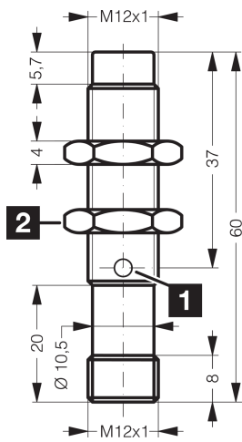
1) LED 2) Width over flats 17 mm BK: black BN: brown BU: blue
