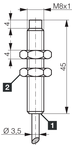
1) LED 2) Width over flats 13 mm BK: black BN: brown BU: blue
