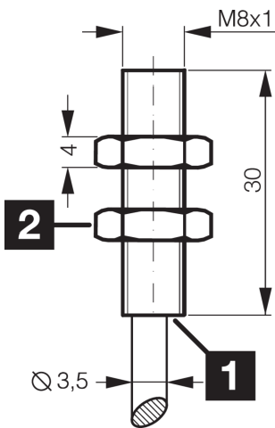
1) LED 2) Width over flats 13 mm BK: black BN: brown BU: blue
