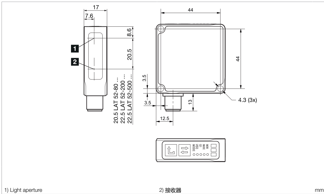
1) Light aperture
